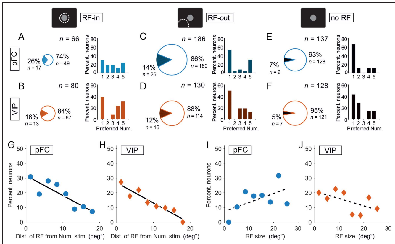
Figure 6. Proportions of numerosity neurons across RF classes. (A) The relative proportions of RF classes in pFC are indicated by the size of the pie charts. The openness of the pie and the shaded area reflect the proportions of numerosity-selective neurons within the class. The percentage and number are written next to the individual pies. These neurons belong to the “RF-in” class. On the right, bar plots show the percentage of numerosity neurons belonging to this RF class that prefer each number. (B) “RF-in” neurons in VIP. The proportion of numerosity-selective neurons in “RF-out” neurons (C) in pFC and (D) in VIP. (E) pFC neurons without a significant RF are the smallest proportion. (F) The proportion of numerosity-selective neurons in VIP “no RF” neurons. (G) The percentage of numerosity selectivity in pFC neurons as a factor of the distance of their RFs (only RF-in and RF-out neurons) from the numerosity stimuli. Each data point is the percentage of selective neurons in that bin; solid line fitted the data to a linear model. Solid lines indicate a significant fit ( p < .01 ). (H) Same as G for VIP neurons. Percentage of numerosity selectivity across RF sizes (I) in pFC and (J) in VIP. Dashed lines indicate fits were not significant ( p > .05 ).
